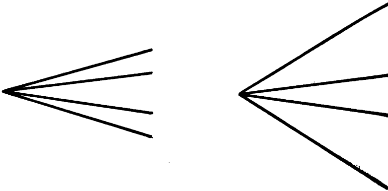
Fig. 20. — Contrasting angles.
